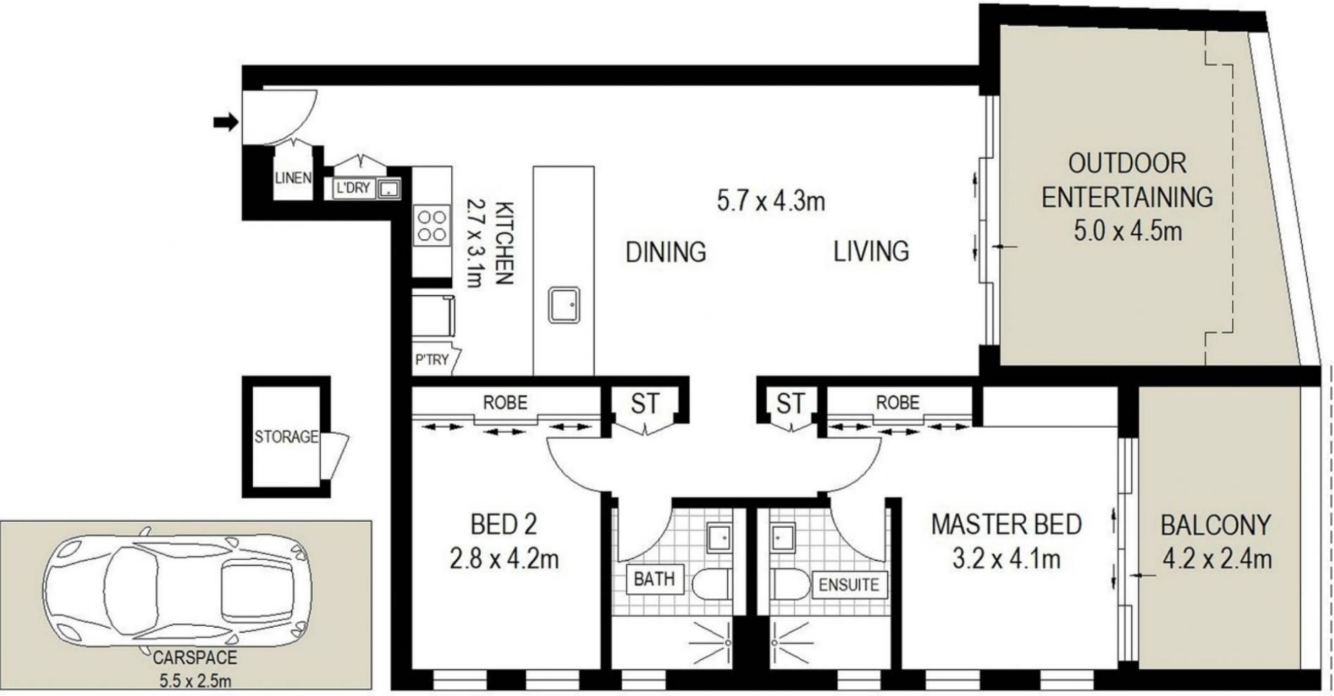
BASEMENT LEVEL
